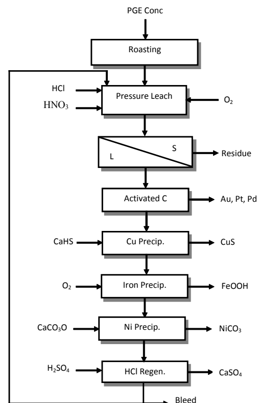
Figure 27. Process Flowsheet for the Treatment of the Lac des Iles PGE Concentrate
