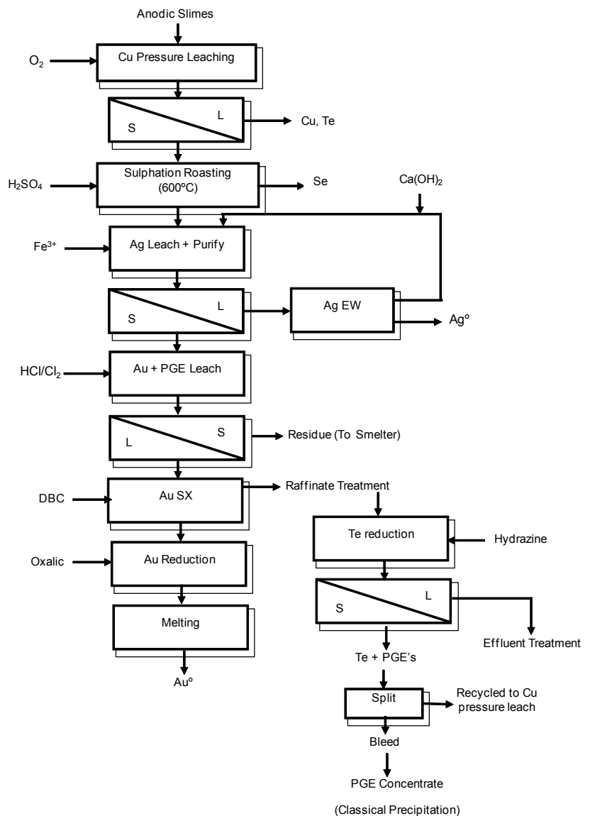
Figure 18. Degussa dmC 2 Process to Recover PGE's from Autocatalysts
