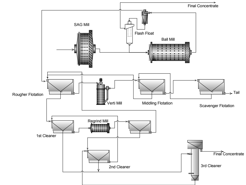
Figure 5. The Lac des Iles Flowsheet
